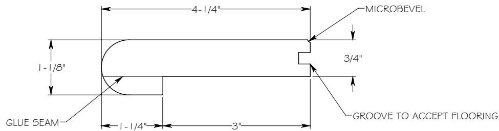
Stair Nose Profile #2 - Built up Bull Nose
