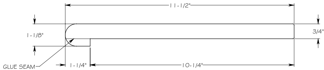
Stair Tread Profile #2 - Built up Bull Nose
